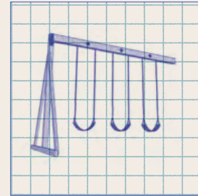
3-Position Swing Beam
